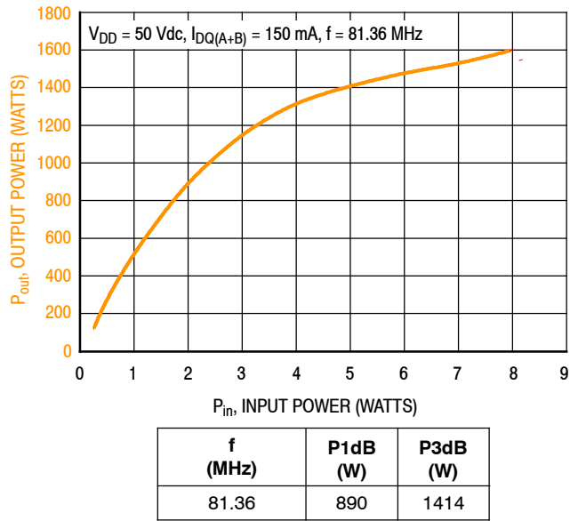
Figure 15. CW Output Power versus Input Power
