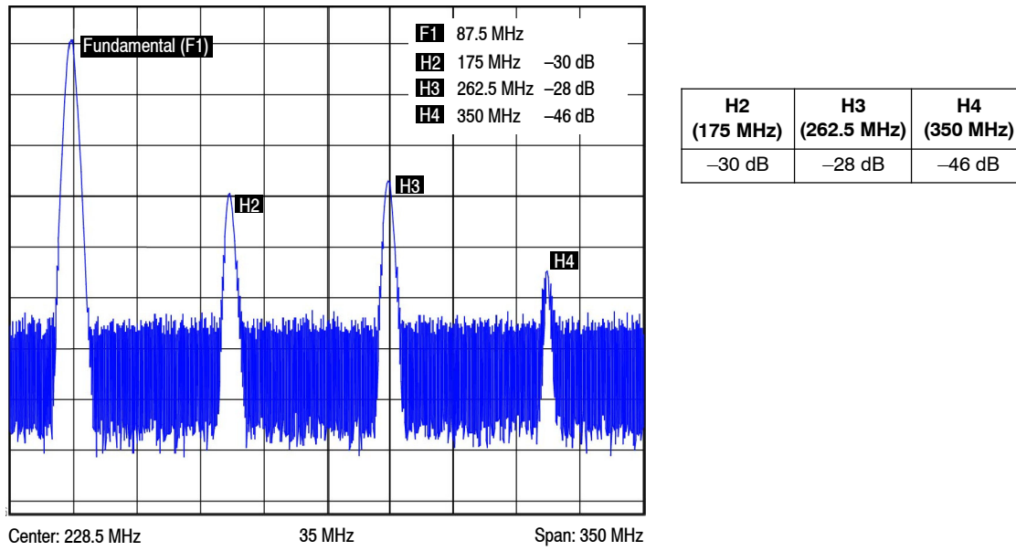
Figure 12. 87.5 MHz Harmonics @ 1200 W CW
